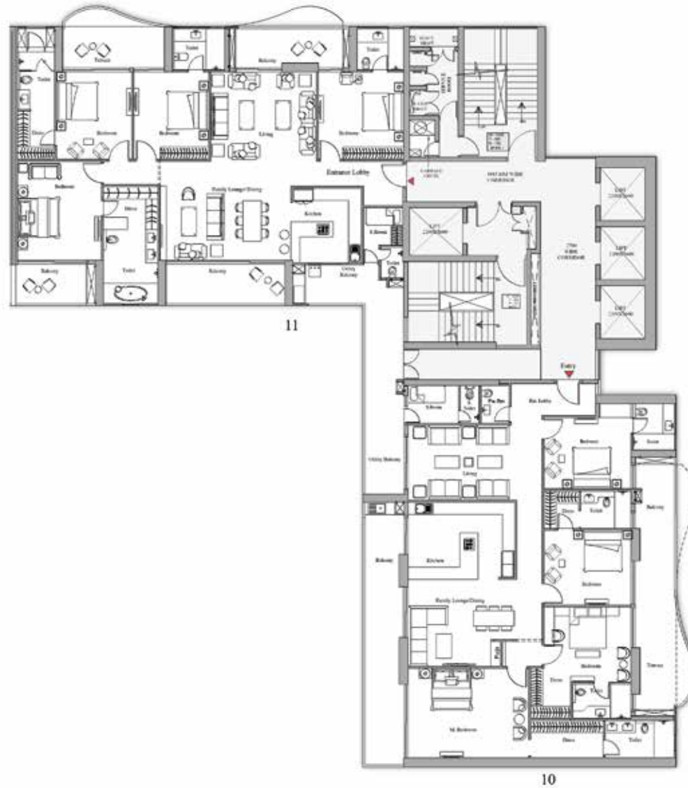
TYPICAL FLOOR PLAN -TOWER(B2)
